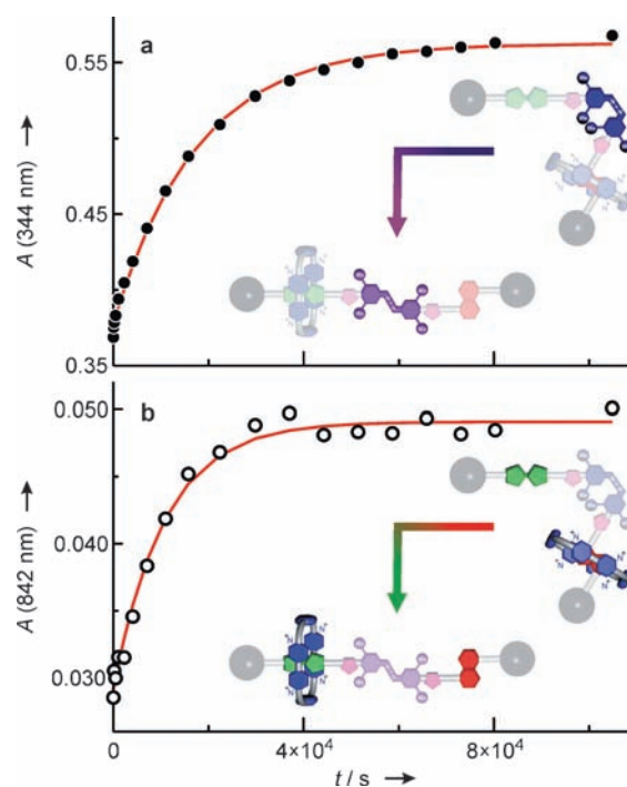
Figure 3. Time-dependent absorption changes (MeCN, 295 K), monitored at a) 344 nm, ( trans -TMeAB absorption) and b) 842 nm (TTF- \text{CBPQT}^{4+} CT absorption), showing the regeneration of \text{trans-1}^{4+} from the metastable state \text{cis-1}^{4+} . The lines represent the data fitting according to a first-order kinetic equation. The corresponding absorption spectra are shown in Figure 2d.
